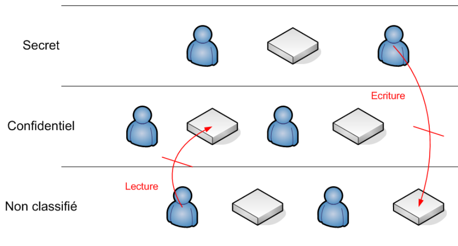
FIG. 2.3 – No Read Up et No Write Down.
